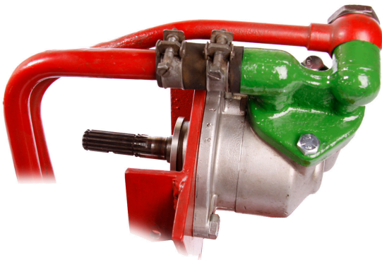
Original design of the hydraulic pump's mounting, seen from the right.
